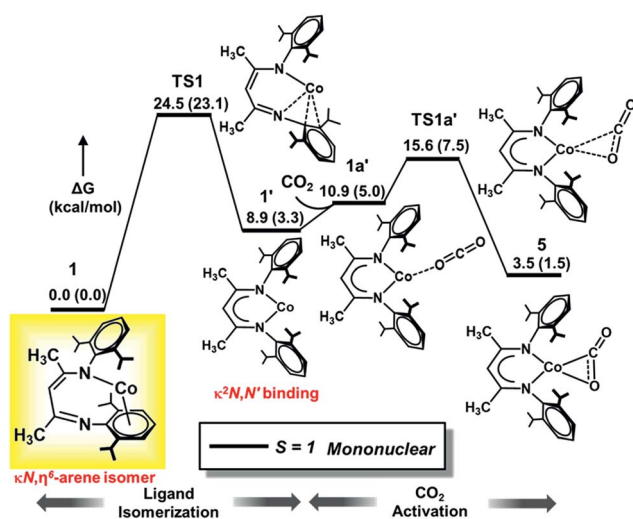
Fig. 4 Computed DLPNO-CCSD(T)/def2-TZVPP Gibbs free energy (ΔG) profile for isomerization of 1 (L'Co) to 1' followed by CO 2 activation. Relative free energy values (in kcal mol -1 ) computed with M06L/def2-TZVPP are given in parentheses. The isolated species is shown in the yellow box, with L' depicted instead of L tBu .
