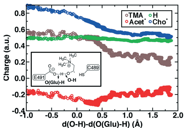
Fig. 8 By-fragment-summed partial charges along the cholanyl radical deprotonation reaction coordinate: total cholanyl radical (Cho • , blue circles) and its substituent transferring H + (green circles), TMA (brown circles), and acetaldehyde radical (Acet • , red circles). A skeleton structure of the distances in the LCOD reaction coordinate is shown in inset.
