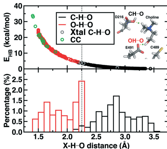
Fig. 9 (top) Hydrogen bond energy ( E_{HB} , in kcal mol −1 ) versus X–H···O distance for i) snapshot MD distances with X=O (red circles), X=C (black circles), ii) all observed close contacts in crystal structures (CC, green circles), and the X=C non-covalent interactions observed in CutC (Xtal C–H···O, gray circles). A snapshot showing the C–H···O and O–H···O hydrogen bond is provided in inset with the BCP shown as a green sphere. (bottom) Normalized distribution of CH···O and OH···O distances from MD snapshots as described for the top pane. A qualitative cutoff between CH···O and OH···O distances is indicated by a vertical dashed line at 2.25 Å.
