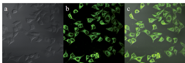
Fig. 9 Fluorescence images of HeLa cells incubated with luminogen 1 (20 µM) for 30 min at 37 °C: (a) bright field image; (b) fluorescence image; (c) merge image (a and b).
