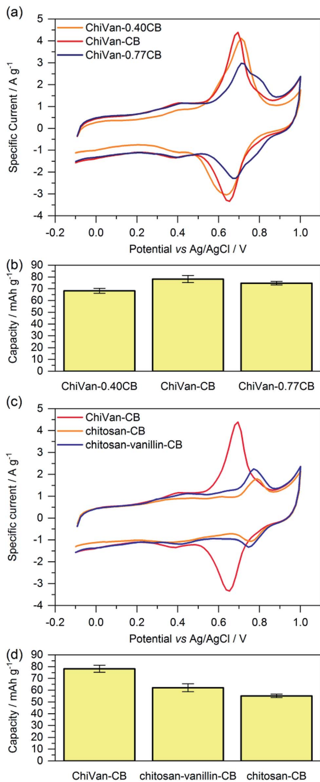
Fig. 4 (a and c) Cyclic voltammograms and (b and d) average capacities as calculated by integration of the cyclic voltammograms of ChiVan-carbon black composites prepared with different ratios of both constituents (a and b) or composites of carbon black with ChiVan or other polymers in which certain steps of the ChiVan synthesis were omitted (c and d). All CV was tested in 1 M HClO 4 aqueous solution (5 mV s -1 ). The fifth cycle of the respective experiment is displayed.
