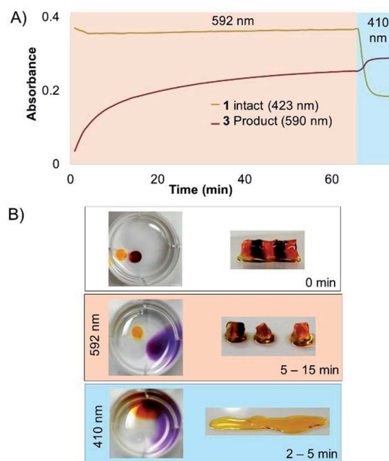
Fig. 6 Selective degradation of 1 and 3 in solution and hydrogel. (A) Irradiation at 592 nm photolyzes 3 while leaving 1 intact, until irradiation at 410 nm. (B) Striped hydrogel incorporating alternating sections of 1 and 3 was selectively degraded at 592 nm, leaving the orange gel regions intact. The remaining sections crosslinked by 1 were degraded by 410 nm light.
