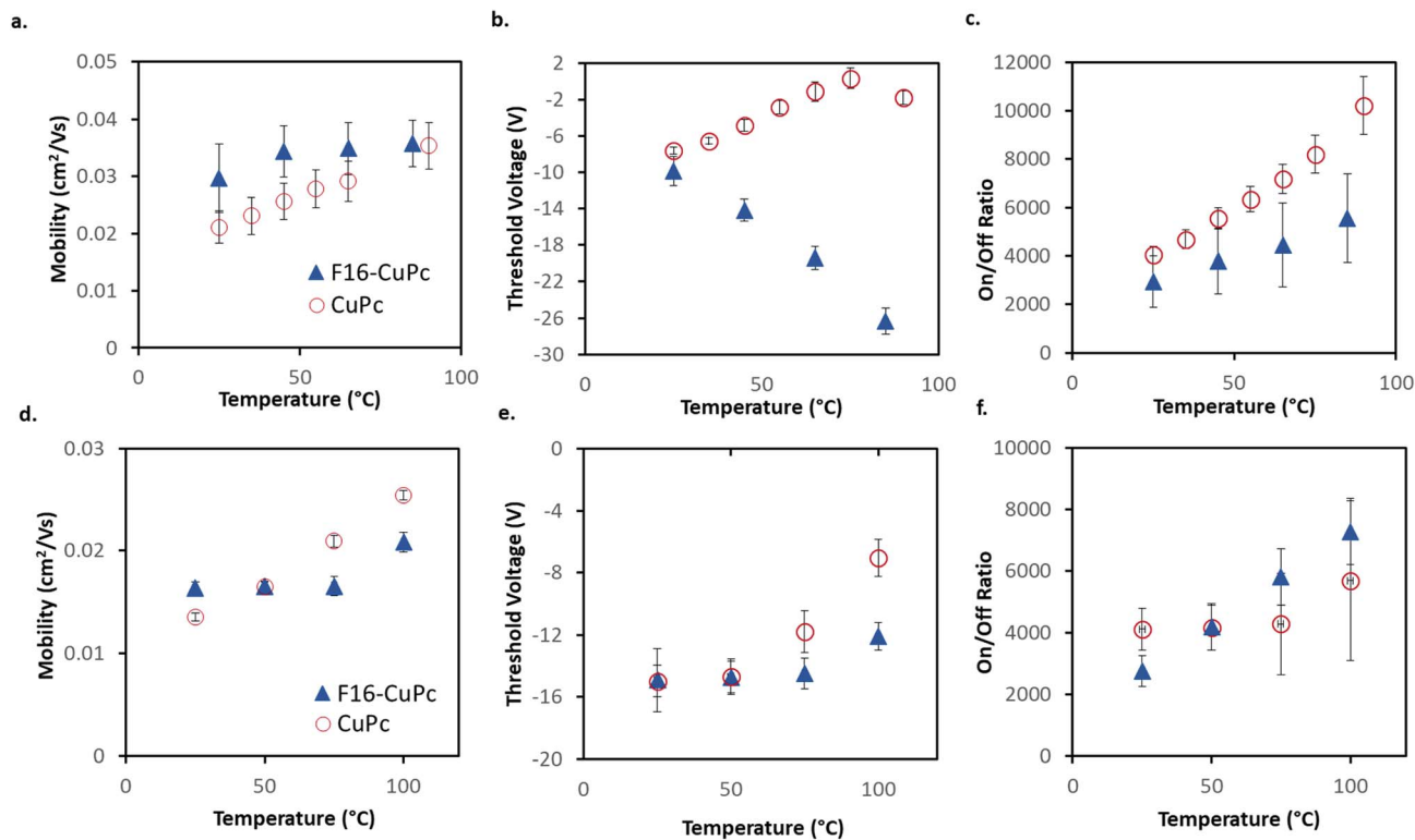
Fig. 4 Performance of BGBC CuPc and \text{F}_{16} -CuPc devices (deposited at T = 140\text{ }^{\circ}\text{C} ) in air (a, b and c) or vacuum (d, e and f) at various temperatures. (a and d) Field-effect mobility. (b and e) Threshold voltage. (c and f) On/off ratio. Presented are the averages for four devices with error bars representing the standard deviation. The legend in (a and d) is the same as in (b and e) and (c and f). Devices were tested in the range of T = 25\text{ }^{\circ}\text{C} to T = 90\text{ }^{\circ}\text{C} in air, and T = 25\text{ }^{\circ}\text{C} to T = 100\text{ }^{\circ}\text{C} in vacuum.
