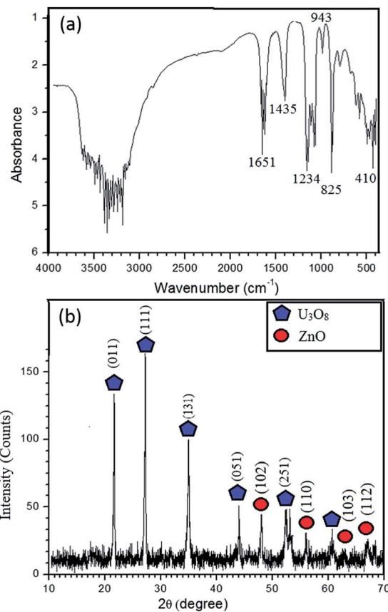
Fig. 1 (a) FT-IR spectrum of UO_2(OH)_2/Zn(OH)_2 . CTAB (b) XRD pattern of the synthesized U_3O_8@ZnO nanocomposite.
