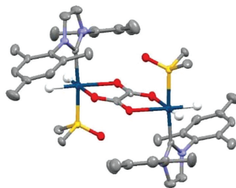
Fig. 5 Structure of [\text{Ir}_2(\text{H})_4(\text{IMes})_2(\text{DMSO})_2(\eta^2\text{-}\kappa^2\text{-Oxalate})] , 6 , determined by X-ray crystallography. All non-hydride hydrogen atoms and solvent of crystallisation have been omitted for clarity.
