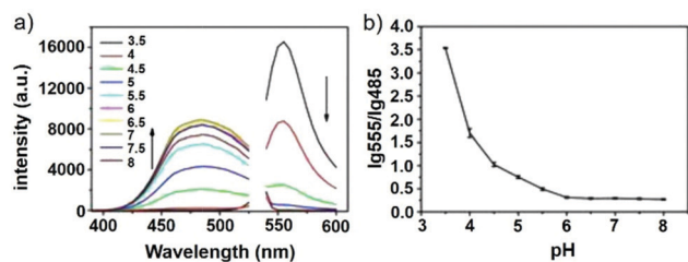
Fig. 19 pH dependent ratiometric fluorescence emission of probe 15 . (a) Fluorescence emission spectra of probe 15 (10 \mu\text{M} ) at pH 3.5–8.0 under dual-wavelength excitation ( \lambda_{\text{exc}} at 300 nm for dansyl group, 532 nm for R6G-lactam). (b) pH titration curves of lg ratios between fluorescence emission of R6G-amide ( I_{555\text{nm}} ) and that of dansyl group ( I_{485\text{nm}} ). Copyright 2013 Elsevier.
