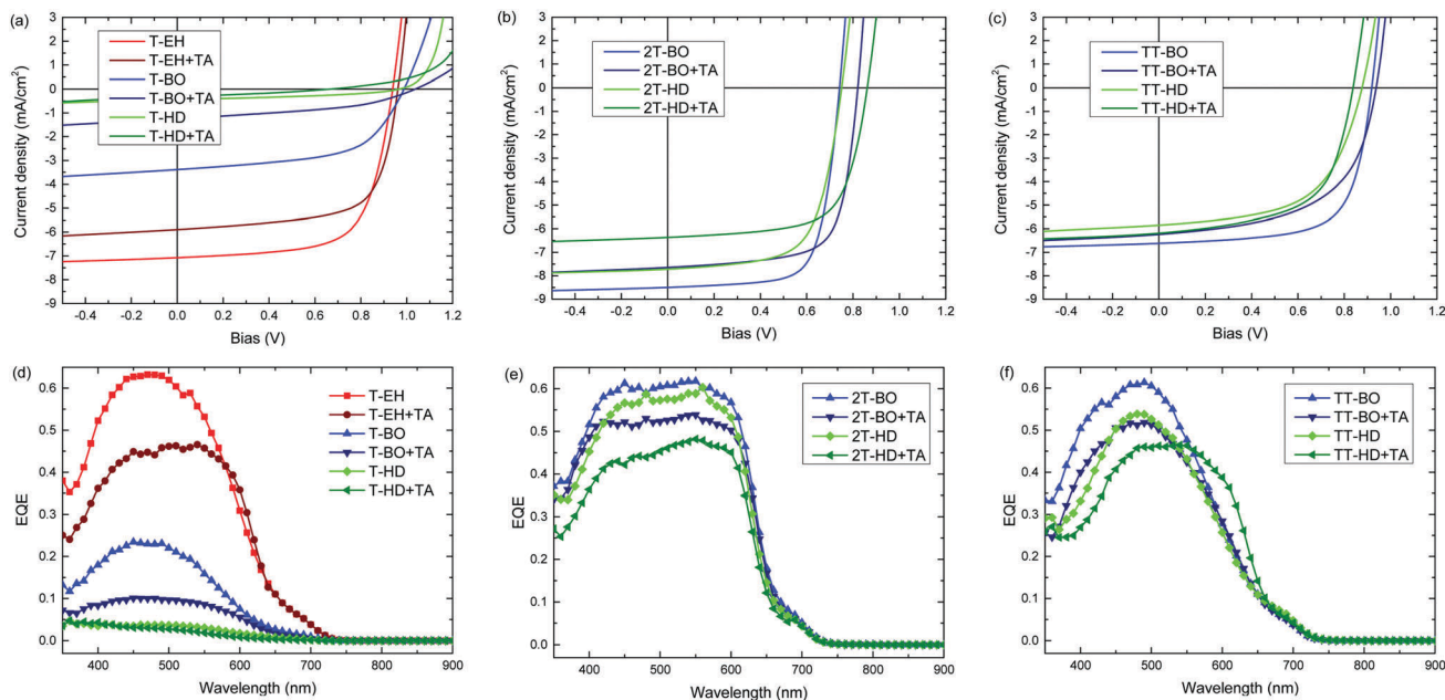
Fig. 4 (a–c) J – V -characteristics of optimized bulk heterojunction solar cells of PDCB polymers containing (a) thiophene, (b), bithiophene, and (c) thienothiophene with PC 71 BM. (d–f) Corresponding EQE spectra of the same devices. TA is thermal annealing for 10 min at 120 °C.
