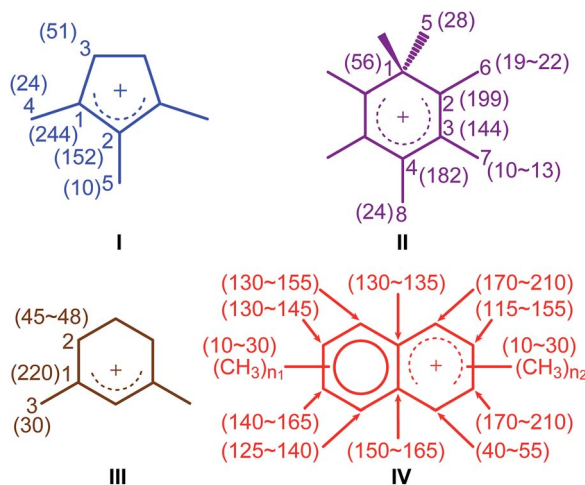
Fig. 2 Carbocations identified in activated M- \beta and MMM- \beta coded with the same colors as their corresponding assignments and correlations in Fig. 3 and 4. Values in the parenthesis are 13 C chemical shifts. n_1 and n_2 are the number of methyl groups with 3 \leq (n_1 + n_2) \leq 7 .
