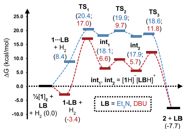
Fig. 5 Computed free energy profile for Et 3 N- and DBU-assisted H 2 activation with 1 . Relative free energies (in kcal mol -1 ) are with respect to 0.5[\mathbf{1}]_2 + \text{LB} + \text{H}_2 .
