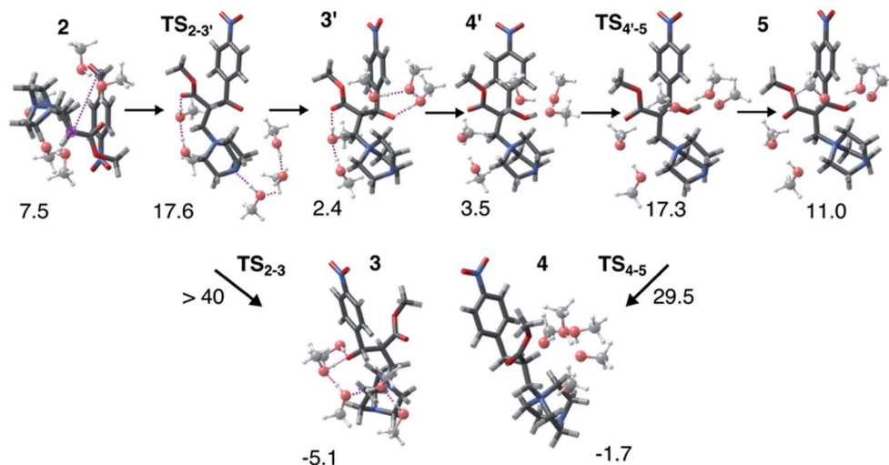
Fig. 5 Structures for the MBH reaction pathway (2 → TS 2-3' → 3' → 4' → TS 4'-5 → 5) highlighting the importance of local solvation stabilizing tautomerizing O groups. Though 3' is calculated to be higher in energy than 3, explicit hydrogen bonding opens a kinetically feasible pathway for C–C coupling. Reaction energies are reported relative to 1.
