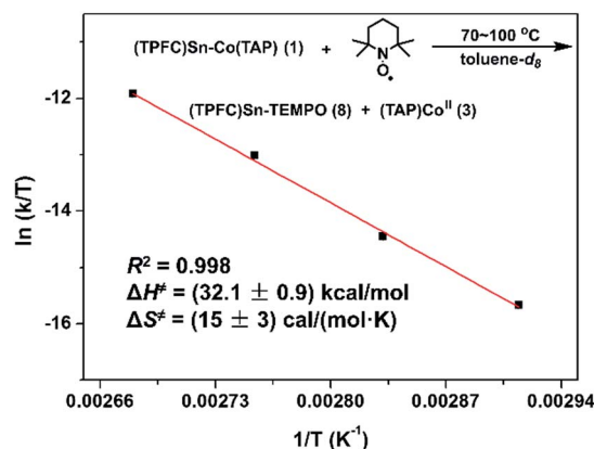
Fig. 9 Eyring plot of the reaction of 1 with TEMPO. Conditions: 1.6 \text{ mmol L}^{-1} of 1 , 16 \text{ mmol L}^{-1} of TEMPO, \text{toluene-}d_8 (containing 15% v/v \text{C}_6\text{D}_6 ), in the dark and under a \text{N}_2 atmosphere.
