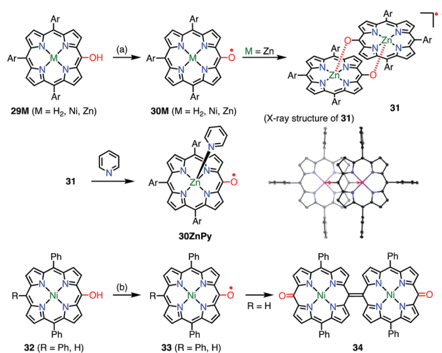
Fig. 11 10,15,20-Triarylporphyrin meso -oxy radicals. (a) 800 equiv. \text{PbO}_2 , \text{CH}_2\text{Cl}_2 , rt, 5 min, 86% for 30H}_2 , 91% for 30Ni , 89% for 31 ; (b) aerobic oxidation for 33 , 7 equiv. DDQ, \text{CH}_2\text{Cl}_2 , rt, 30 min, 26% for 34 . Ar = 3,5-di- tert -butylphenyl. Hydrogen atoms and tert -butyl groups in the crystal structure of 31 were omitted for clarity.
