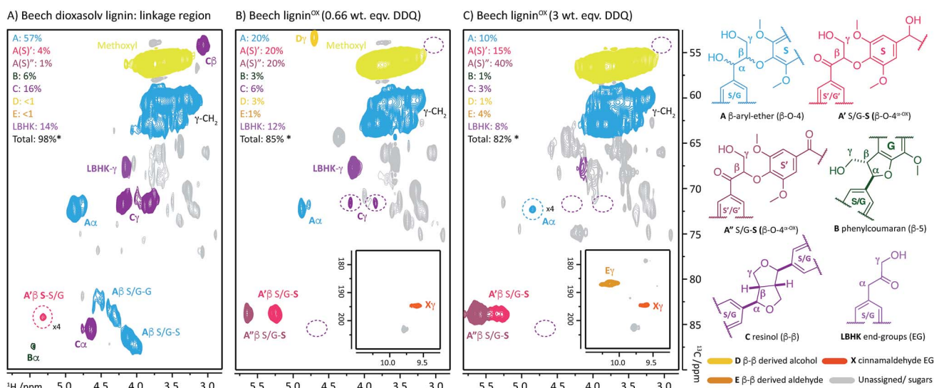
Fig. 2 2D HSQC NMR analysis (700 MHz, d_6\text{-DMSO} ) of: (A) beech dioxasolv lignin linkage region; (B) beech lignin ^{\alpha-\text{OX}} post reaction with 0.66 wt equiv. of DDQ and; (C) with 3 wt equiv. of DDQ. Percentages were calculated assuming the units present are 100% of the linkage content and are based on semi-quantitative analyses of lignin samples. 38 For an example of integral analysis see Fig. S5.† For full raw data see Table S3 and Fig. S6.† Assignments of key structures are based on data from this study and the literature. 5,8,26,30,39–44 \gamma\text{-CH}_2 assigned cross-peak refer to all possible alkyl-oxygenated \text{CH}_2 -groups present in the lignin chain. Threshold levels in the analysis of the 2D HSQC NMR have been lowered to observe key cross-peaks. The oxidation of G- \beta\text{-O-4} structures is discussed in more detail in the ESI.† *Total percentage of linkages < 100% due to omission of A'/A'' S/G-G ( \beta\text{-O-4}^{\alpha-\text{OX}} ) values, please see Table S3 for further details.†
