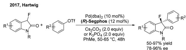
Scheme 31 Pd-catalyzed enantioselective \alpha -arylation of \alpha -fluorooxindoles.
