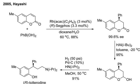
Scheme 3 The enantioselective 1,4-addition of arylboronic acids to \beta -aryl substituted unsaturated carbonyl derivatives.
