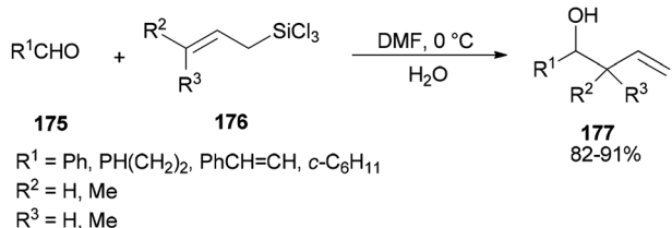
Scheme 88 Synthesis of the desired syn - and anti -homoallylic alcohols 177.
