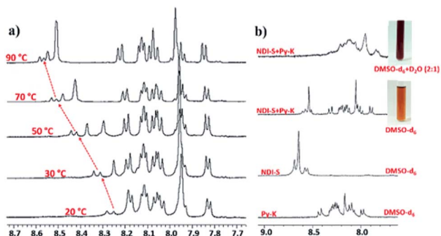
Fig. 4 (a) Temperature dependent ^1\text{H} NMR spectra 1a + 2d in \text{DMSO-d}_6 : \text{D}_2\text{O} (2 : 1); (b) solvent dependent ^1\text{H} NMR spectra of 1a , 2d and 1a + 2d . Inset images showing the colour of 1a + 2d mixture in different solvents.
