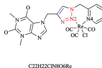
Scheme 28 Structures of the \text{C}_{17.25}\text{H}_{13}\text{ClN}_4\text{O}_{3.25}\text{Re} , \text{C}_{19}\text{H}_{18}\text{ClN}_4\text{O}_4\text{Re} , and \text{C}_{22}\text{H}_{22}\text{ClN}_8\text{O}_6\text{Re} complexes.
