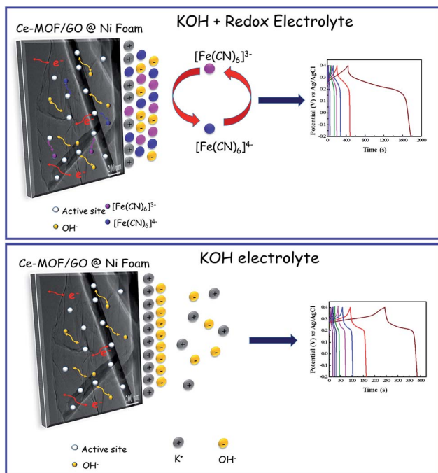
Fig. 9 Charge transport mechanism of Ce-MOF/GO composite.
