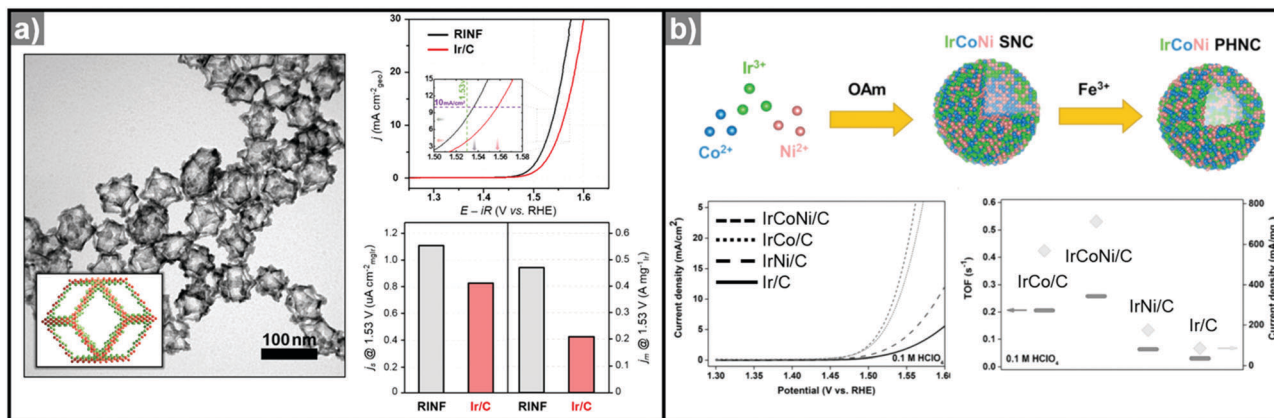
Fig. 12 (a) TEM image of IrNi nanostructure with graphical model in the inset and comparison of its OER activity with Ir/C (right; up). Specific activity and mass activity of IrNi nanostructure and commercial Ir/C are compared at 1.53 V (right; down). Reproduced with permission from ref. 294. Copyright 2017 Elsevier. (b) Scheme for the synthesis of IrCoNi multimetallic porous hollow nanocrystals and comparison of their OER activities (down; left) and turnover frequency (TOF) values and current densities of OER normalized to the mass of Ir (down right). Reproduced with permission from ref. 296. Copyright 2017 Wiley-VCH.
