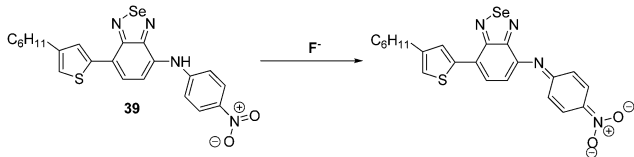
Scheme 36 A benzoselenadiazole-based diarylamine ESPIPT fluorescent probe 39 . This system permits detection of the fluoride as the result of a deprotonation event. Measurement conditions: DMSO.
