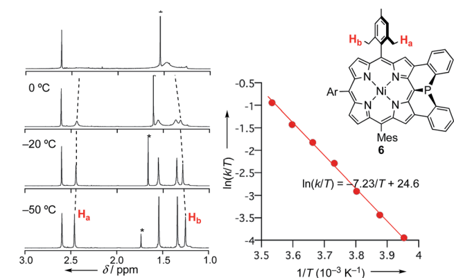
Fig. 2 Temperature-dependent ^1\text{H} NMR spectra of 6 in \text{CDCl}_3 , and Eyring plot for determination of the pyramidal inversion barrier of the phosphorus center.
