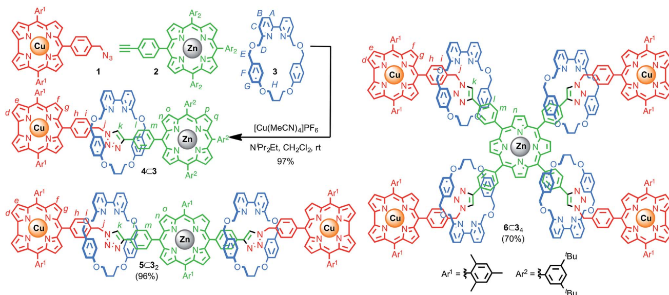
Scheme 1 Synthesis of dyad 4C3 and structures of triad [3]rotaxane 5C3 2 and pentad [5]rotaxane 6C3 4 .
