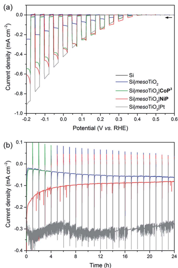
Fig. 3 (a) LSVs of Si (black), Si|mesoTiO 2 (blue), Si|mesoTiO 2 |CoP 3 (green), Si|mesoTiO 2 |NiP (red) and Si|mesoTiO 2 |Pt (grey) electrodes under chopped illumination ( v = 5 \text{ mV s}^{-1} ). (b) CPP traces for Si|mesoTiO 2 , Si|mesoTiO 2 |NiP, Si|mesoTiO 2 |CoP 3 and Si|mesoTiO 2 |Pt electrodes (see (a) for colour-coding) at E_{\text{app}} = 0.0 \text{ V vs. RHE} under continuous illumination with an hourly dark chop lasting for two min each. Conditions: aqueous acetic acid solution (0.1 M, pH 4.5), UV-filtered simulated solar light irradiation (AM1.5G, 100 mW cm -2 , \lambda > 400 \text{ nm} ), N 2 atmosphere, room temperature.
