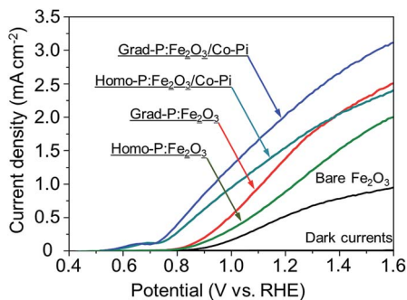
Fig. 4 I - V characteristics of bare Fe 2 O 3 , homo-P:Fe 2 O 3 , grad-P:Fe 2 O 3 , homo-P:Fe 2 O 3 /Co-Pi and grad-P:Fe 2 O 3 /Co-Pi photoanodes measured in 1 M KOH solution under AM 1.5G illumination (100 mW cm -2 ). The dark currents are negligible for all samples.
