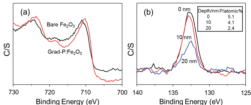
Fig. 3 (a) XPS spectra of the Fe 2p signal in bare Fe 2 O 3 and grad-P:Fe 2 O 3 photoanodes; (b) XPS depth profile signal of P 2p in grad-P:Fe 2 O 3 , where the P concentration decreases with increasing sputtering time (inset shows the P atomic concentration values at different depth).
