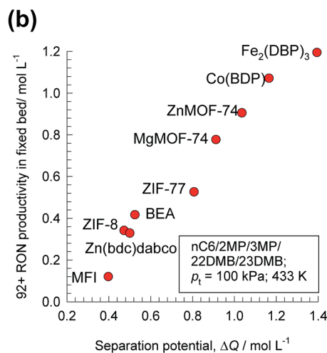
Fig. 9 (a) Transient breakthrough simulations for separation of equimolar nC6/2MP/3MP/22DMB/23DMB mixtures at 433 K and 100 kPa in fixed bed adsorber packed with MgMOF-74. Also shown is the RON of product gas at the outlet of fixed bed. (b) Comparison of 92+ RON productivity for operation at total pressure of 100 kPa, plotted as a function of the separation potential \Delta Q_{(22DMB+23DMB)/(nC6+2MP+3MP)} , calculated from eqn (19) and IAST. All calculation details and structural information on the various MOFs are provided in the ESI.†
