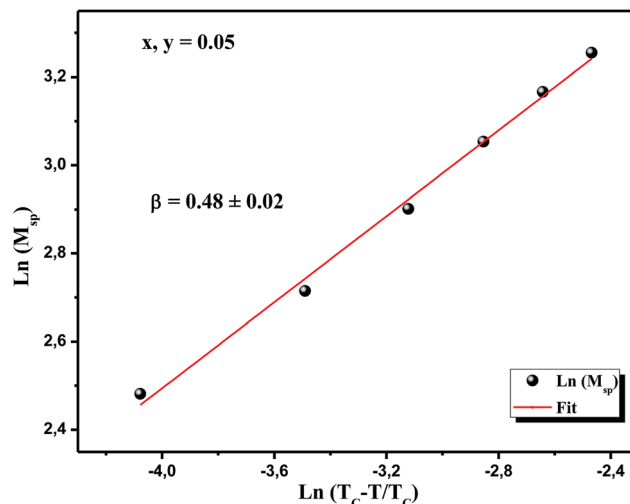
Fig. 15 \ln(M_{sp}) vs. \ln(T_C - T/T_C) . The red line is the linear fitting.
