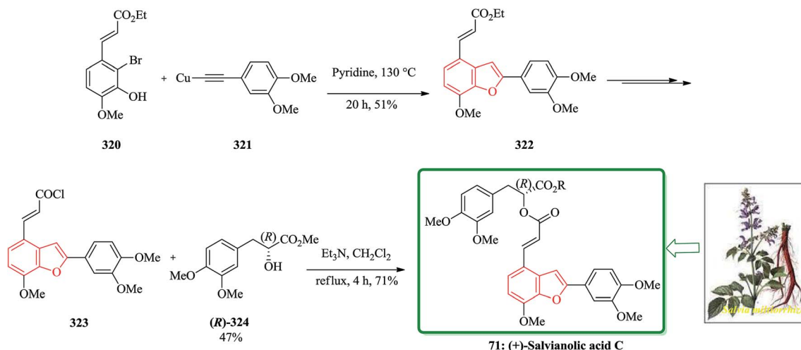
Scheme 70 Total synthesis of (+)-salvianolic acid 71 .
