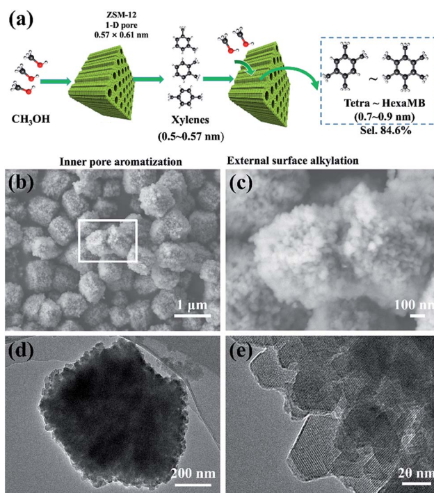
Fig. 1 (a) Proposed technical route for the preparation of multi-methylbenzenes from methanol using a nano ZSM-12 zeolite-based catalyst. (b) SEM image of H-ZSM-12. (c) High-resolution SEM image of H-ZSM-12. (d) TEM image of H-ZSM-12. (e) High-resolution TEM image of H-ZSM-12.
