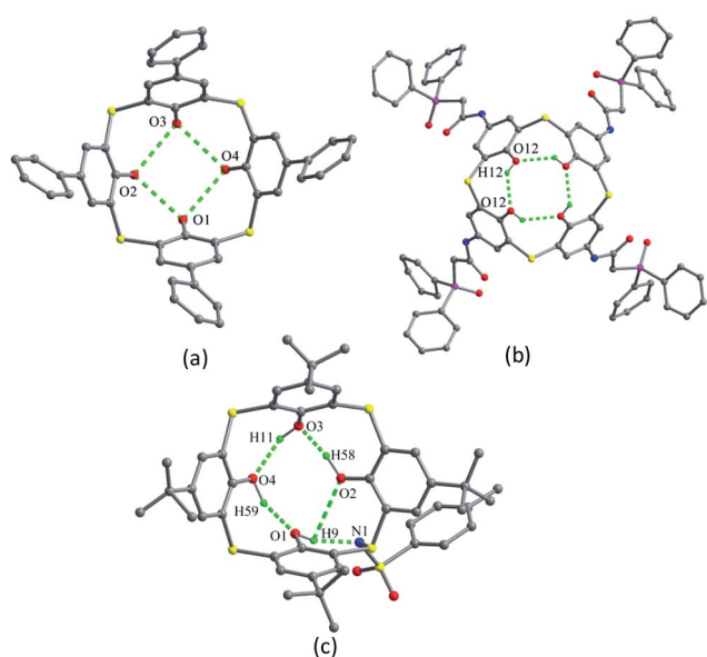
Fig. 7 Crystal structures of 6 (a), 7 (b) and 8 (c), showing the circular H-bonding array.
