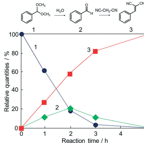
Fig. 6 Time course of the one-pot deacetalization–Knoevenagel condensation reaction over \text{Fe}_3\text{O}_4@HKUST-1 ; benzaldehyde dimethylacetal (1, ●), benzaldehyde (2, ◆), benzylidene-malononitrile (3, ■).
