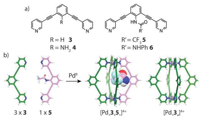
Fig. 5 (a) Endohedrally functionalized ligands 3–6 bearing varying degrees of steric bulk; (b) integrative self-sorting of ligands 3 and 5 to give a 3 : 1 mixture of [Pd 2 3 3 5] 4+ and [Pd 2 3 4 1] 4+ . The NHCOCF 3 endohedral substituent in the heteroleptic assembly is shown as a space-filling representation.
