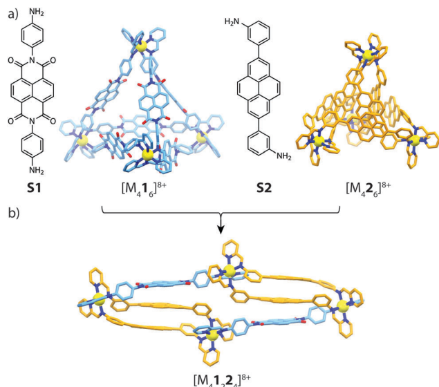
Fig. 4 (a) Electron-poor ( S1 ) and electron-rich ( S2 ) sub-components and their respective homoleptic assemblies; (b) the heteroleptic [M 4 1 2 2 4 ] 8+ product (M = Fe II , Co II , Zn II ).
