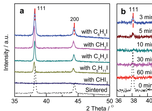
Fig. 1 (a) XRD patterns of sintered Au/C catalyst and after treatment with various iodohydrocarbons 40\text{ }^\circ\text{C} for 3 h; (b) XRD patterns of sintered Au/C catalyst before and after treatment with \text{CHI}_3 at 40\text{ }^\circ\text{C} as a function of time.
