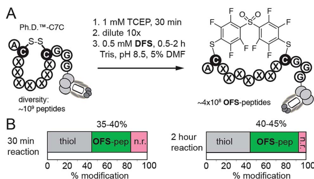
Fig. 5 (A) An aqueous solution of DFS containing 5% DMF as co-solvent can conveniently convert commercially available phage displayed library of 10 9 disulfide heptapeptides—Ph.D. ™ -C7C from New England Biolabs—to a library of OFS -macrocyclic peptides. (B) Biotin capture, analogous to that described in Fig. 4C–E, quantified the efficiency of this modification. After 30 minutes to 2 hours reaction with DFS , 35–45% of the library is modified with DFS yielding ~350–450 million of diverse phage-displayed OFS -macrocycles. Data is averaged from two independent experiments.
