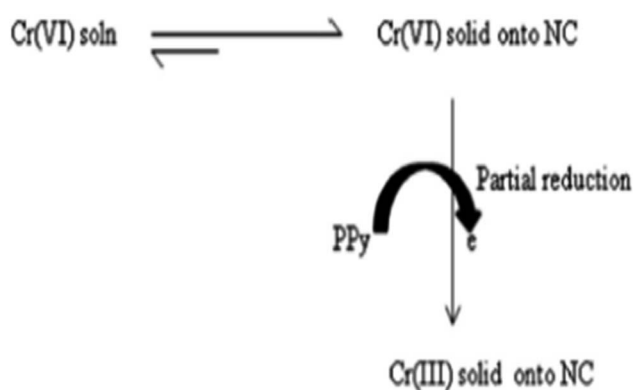
Scheme 5 The mechanism for adsorption and partial reduction of Cr(VI) onto the PPy-OMMTNC nanocomposite. 123
