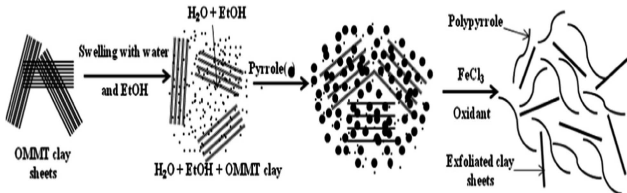
Fig. 7 The formation of exfoliated PPy-OMMTNC nanocomposites. 123
