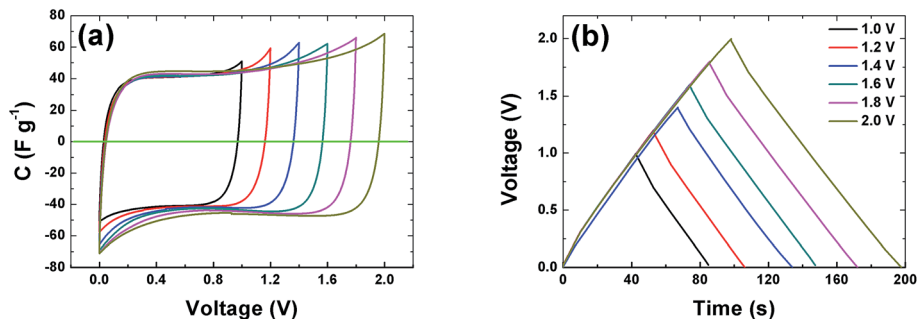
Fig. 6 (a) Cyclic voltammogram at 20 \text{ mV s}^{-1} and (b) galvanostatic charge–discharge profiles of the APC at 0.5 \text{ A g}^{-1} at different voltage ranges respectively.
