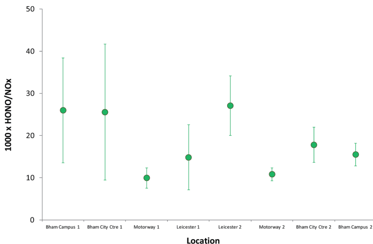
Fig. 11 Mean ( \pm 1 standard deviation) HONO/ \text{NO}_x ratios observed for each environment, spatially defined, during the on-road transect measurements.
