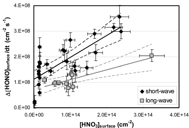
Fig. 5 HONO flux density as a function of the measured surface concentration of HNO 3 using two different sets of UV lamps (~42–57% r.h.). The straight lines represent linear regressions of the data with their 95% confidence limits (dashed lines).
