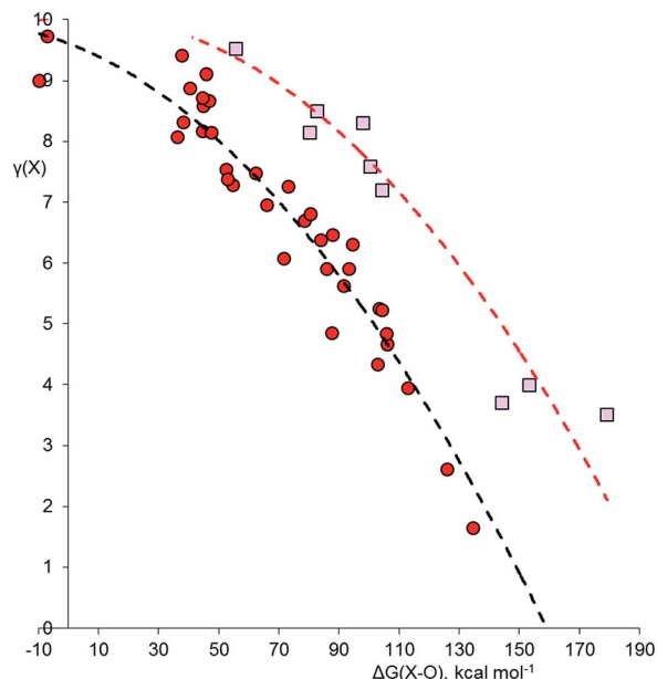
Fig. 3 Plot of \gamma(X) versus \Delta G(X-O) for oxides XO_n^{m-} . Points for second row and heavier elements are represented by pink squares and red circles respectively. The dashed curves are an empirical fit to the two data sets, offset by 43.5 \text{ kcal mol}^{-1} to the right for the second row elements. Correction factors; -9.6 and +56.2 \text{ kcal mol}^{-1} for explicit and implicit Rb^+ respectively.
