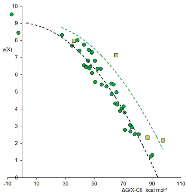
Fig. 2 Plot of \gamma(X) versus \Delta G(XCl) for chlorides XCl_n^{m-} . Points for second row and heavier elements are represented by light green squares and dark green circles respectively. The dashed curves are an empirical fit to the two data sets, offset by 12.7 \text{ kcal mol}^{-1} to the right for the second row elements. Correction factors; -20.2 and +25.4 \text{ kcal mol}^{-1} for explicit and implicit Rb^+ respectively.
