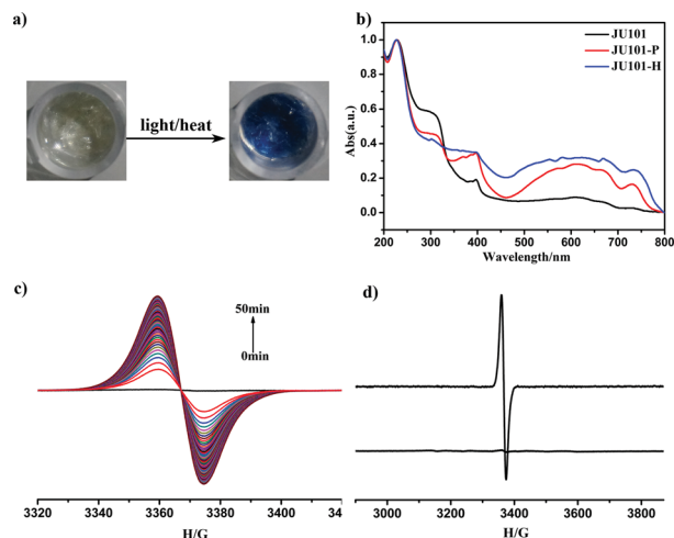
Fig. 2 (a) Photo-/thermochromic phenomenon of JU101. (b) UV/Vis spectra of JU101, photo irradiated sample JU101-P, and heated sample JU101-H. (c) In situ time dependent EPR spectra of JU101 by UV irradiation. (d) EPR spectra of JU101 and JU101-H.
