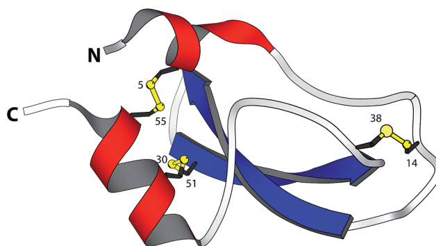
Fig. 1 Structure of BPTI. The folded protein contains three native disulfide bonds between cysteines 5–55, 14–38, and 30–51 (PDB entry: 1BPI).
