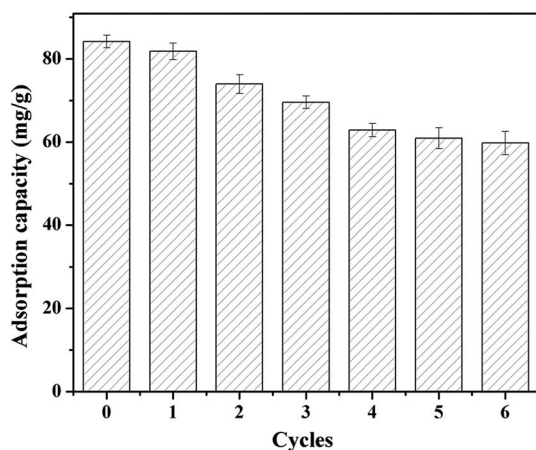
Fig. 13 Sixth consecutive adsorption-desorption cycles of zinc-biochar for Cr(vi) removal (volume: 50 mL; adsorbent dose: 0.1 g; initial Cr(vi) concentration: 500 mg L ^{-1} ; pH: 2.0; contact time: 24 h).
