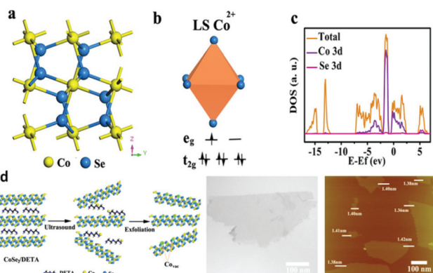
Fig. 11 (a) Crystal structure of \text{CoSe}_2 in the cubic pyrite-type phase; (b) schematic spin structure of the Co cation; (c) DOS diagram for \text{CoSe}_2 ; (d) schematic of the formation of V''_{\text{Co}} vacancies in \text{CoSe}_2 ultrathin nanosheets (left), TEM image (middle) and AFM image (right) of the ultrathin \text{CoSe}_2 nanosheet (reproduced with permission from ref. 43. Copyright 2014 American Chemical Society).
