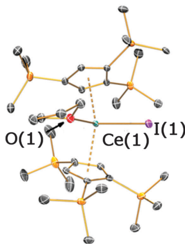
Fig. 6 Molecular structure of 5 with selective atom labelling, with displacement ellipsoids set at the 50% probability level; hydrogen atoms have been omitted for clarity. Selected bond distances [Å] and angles [°] for 5 : Ce(1)–I(1) 3.1000(4), Ce(1)–O(1) 2.490(3), Ce(1)···Cp centroid (1) 2.5416(16), Ce(1)···Cp centroid (2) 2.5259(19), I(1)–Ce(1)–O(1) 89.01(7), Cp centroid (1)–Ce(1)–Cp centroid (2) 133.77(6).
