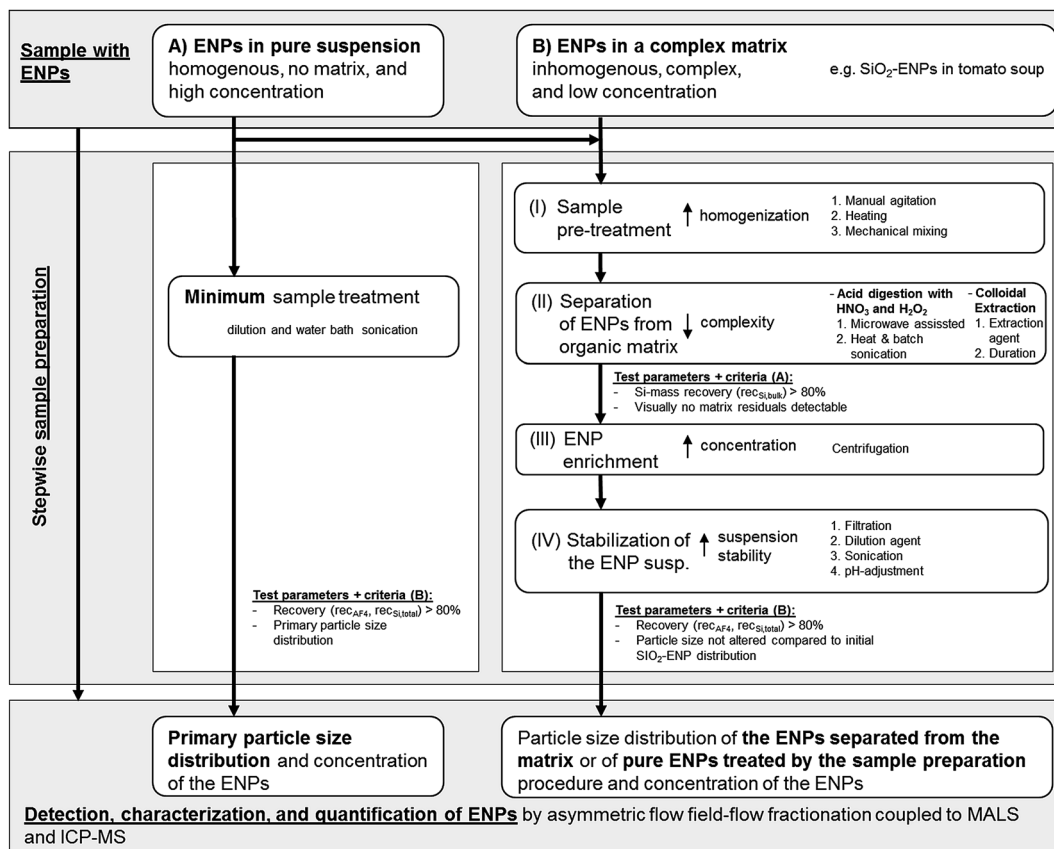
Fig. 1 Generic multi-step procedure for development of a sample preparation method to extract ENPs from a complex matrix. Specific details for the example separation of \text{SiO}_2 -ENPs from tomato soup are given on the right side of the scheme (numbered sub-steps can be performed as stand-alone or in combination with other listed sub-steps).
