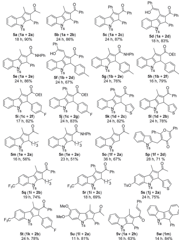
Reaction scheme for the synthesis of indole derivatives 1a-h and 1i-m via a one-pot process: Starting materials: 1a-h (R-substituted 2-alkynyl-1-phenyl-1H-imidazoles) and 1i-m (R-substituted 2-alkynyl-1-phenyl-1H-imidazoles). Reaction conditions: 1a-h : AuCl (2 mol%), K 2 CO 3 (2 mol%), DCE, 60 °C, 1,3-dicarbonyl (1.1 equiv), TIOH (10 mol%), DCE, 60 °C. 1i-m : AuCl (2 mol%), K 2 CO 3 (2 mol%), DCE, 60 °C, 1,3-dicarbonyl (1.1 equiv), TIOH (10 mol%), DCE, 60 °C. Products: 1a-h : Indole derivatives with R-substituents. 1i-m : Indole derivatives with R-substituents. Reaction scheme for the synthesis of indole derivatives 2a-m via a one-pot process: Starting materials: 2a-m (R-substituted 2-alkynyl-1-phenyl-1H-imidazoles). Reaction conditions: 2a-m : AuCl (2 mol%), K 2 CO 3 (2 mol%), DCE, 60 °C, 1,3-dicarbonyl (1.1 equiv), TIOH (10 mol%), DCE, 60 °C. Products: 2a-m : Indole derivatives with R-substituents.
