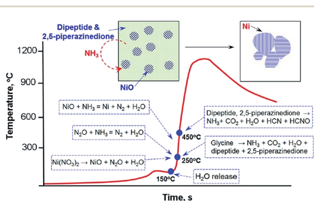
Fig. 2 A schematic illustration showing the mechanism of Ni formation during self-sustained combustion reactions of nickel nitrate–glycine gels. 74 Adopted from ref. 74, Copyright 2013, with permission from American Chemical Society.
