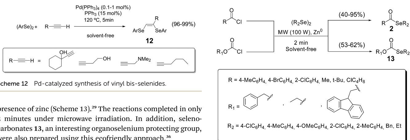
Scheme 13 Solvent-free synthesis of seleno-esters and selenocarbonates.
